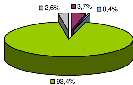
NH 3
