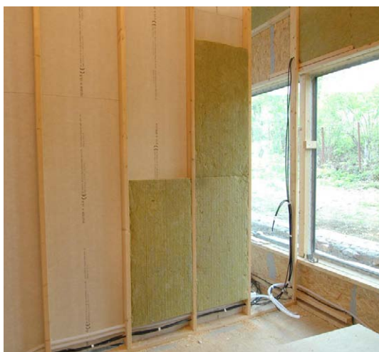
Fig. 1 - Example of use ISOVER Orsik
