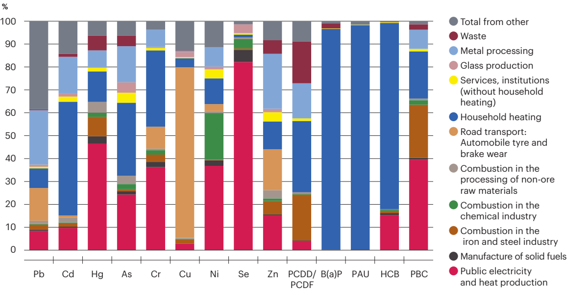
Chart 5 Sources of air emissions of selected heavy metals and POPs in the Czech Republic [%], 2019
